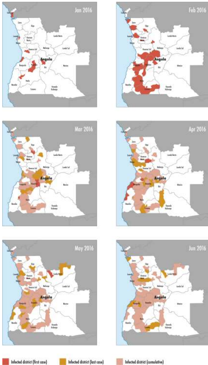
Figure 6. Geographic evolution of the yellow fever epidemic in Angola — monthly snapshots between January and June 2016
