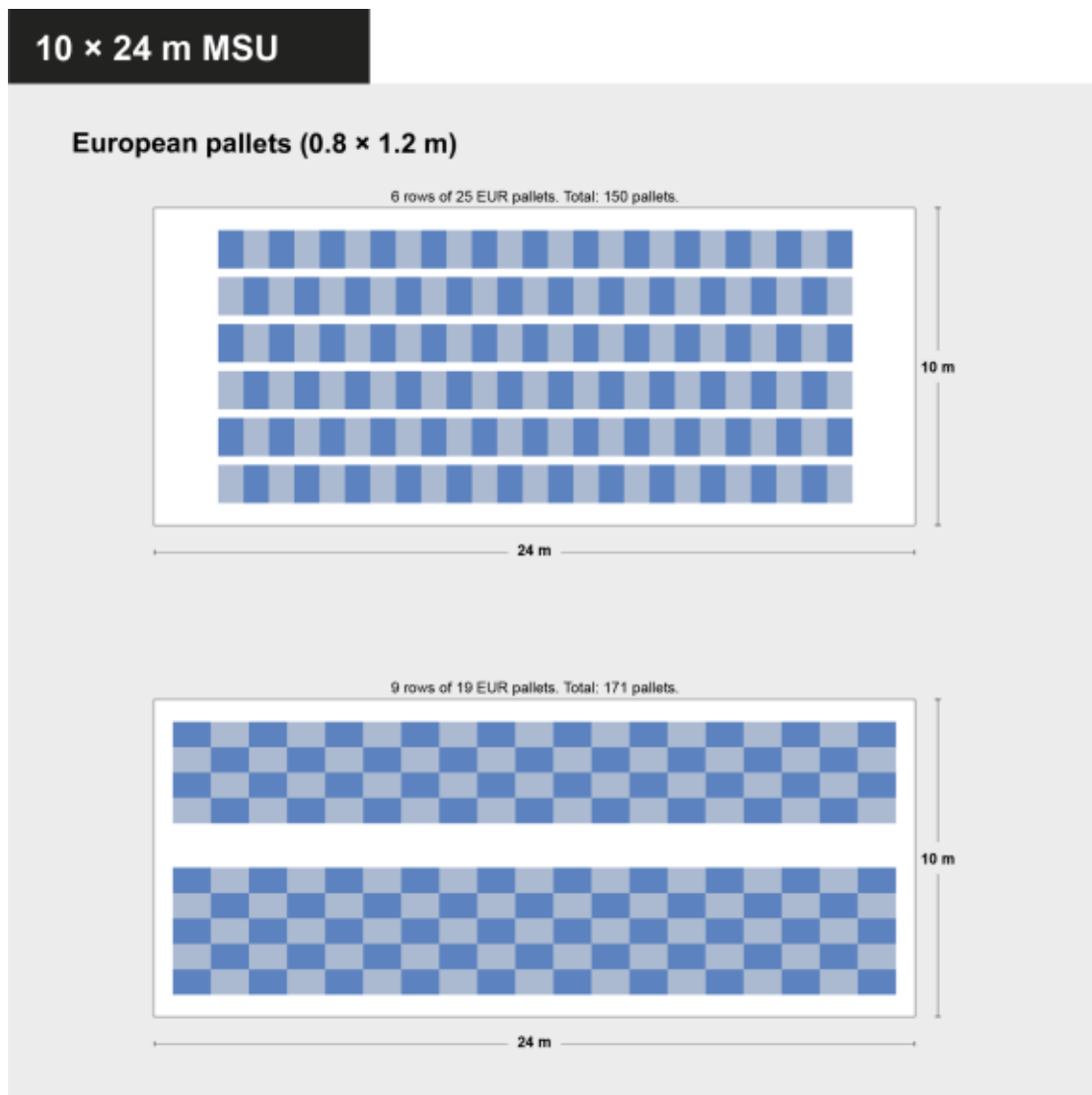
Figure 10. 10 \times 24 m MSU: European pallet configurations
