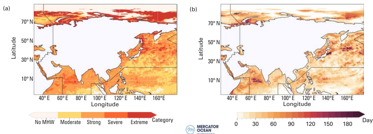
Figure 15. (a) Maximum categories of MHWs and (b) maximum duration of MHWs in 2023. Colours in (a) indicate the highest category of MHW for the year 2023 at each grid point and colours in (b) indicate the duration of MHW at the highest level for each grid point.
